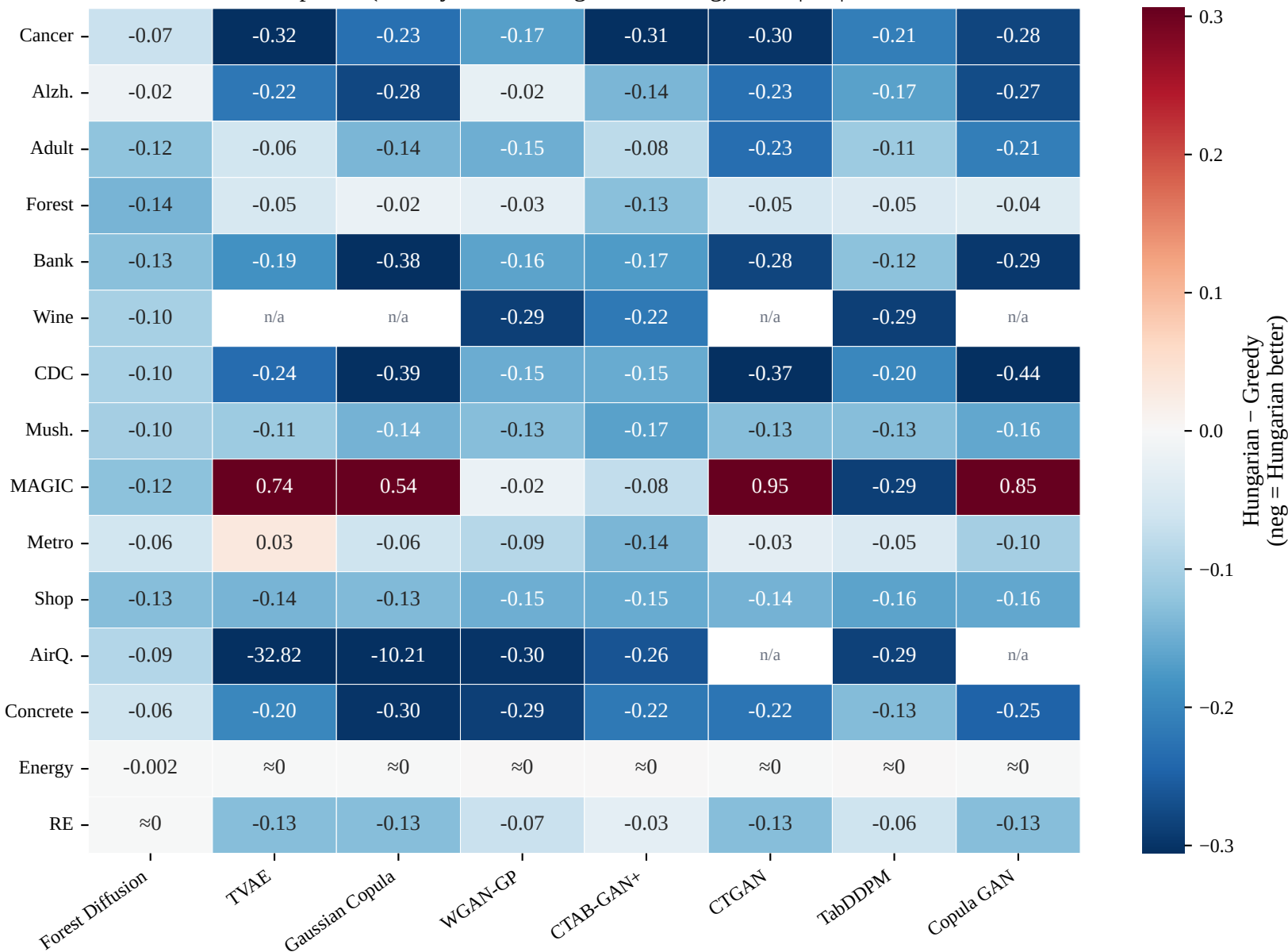
Mahalanobis difference heatmap (Hungarian – Greedy) n/a = unpaired (Greedy and/or Hungarian missing); \approx 0 = |\text{diff}| < 5 \times 10^{-4}
